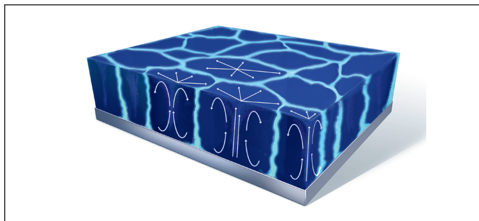
Figure 12: When drying, the surface tension of a coating can be locally very different (surface tension gradient). Turbulence inside the liquid coating leads to areas with higher and lower surface tension
