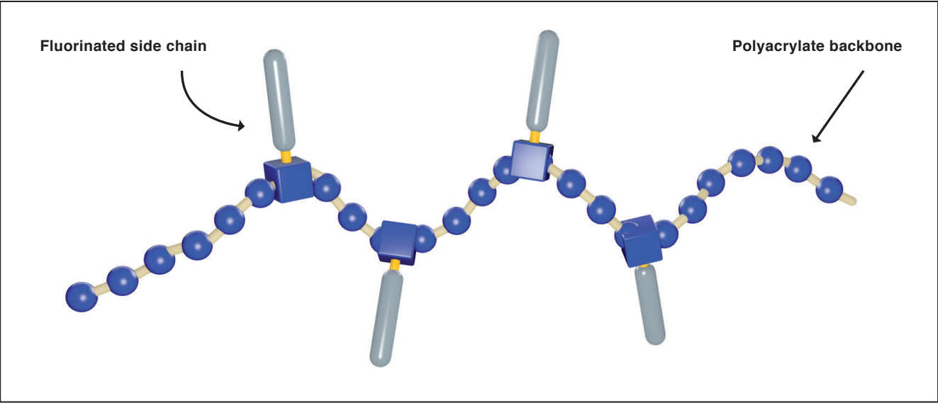
Figure 17: General chemical structure of a fluorocarbon-modified polyacrylate
