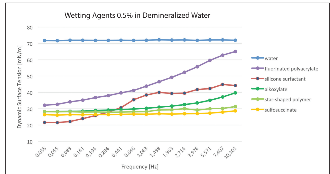
Figure 7: Dynamic surface tension at different bubble frequencies of various wetting agents in water
