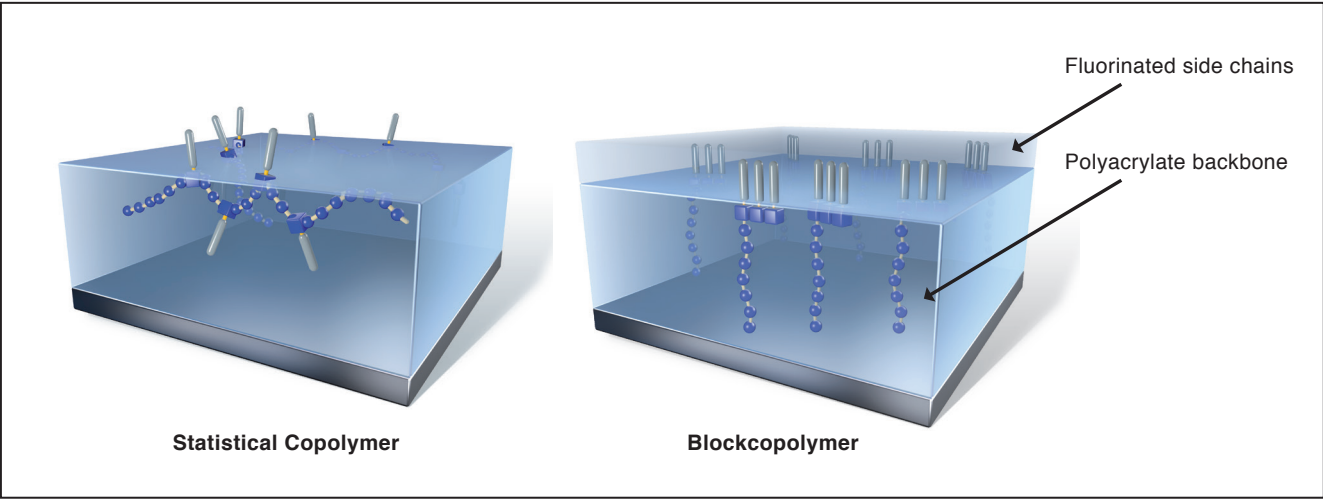
Figure 18: Illustration of a fluorinated polyacrylate at the liquid/air interface. The block copolymer arrangement makes maximum use of the fluorinated side chains
