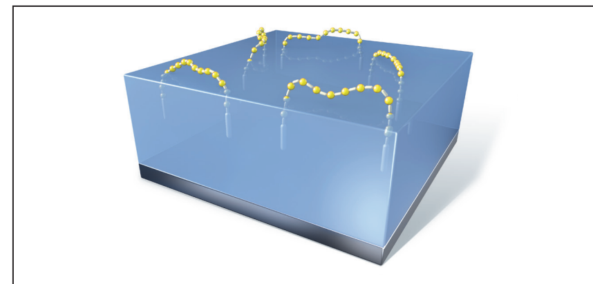
Figure 13: Orientation of organomodified silicones at the surface of a coating. Silicone chains (yellow) orient themselves at the liquid/air interface, whereas the organic side chains have a good compatibility with the coating matrix
