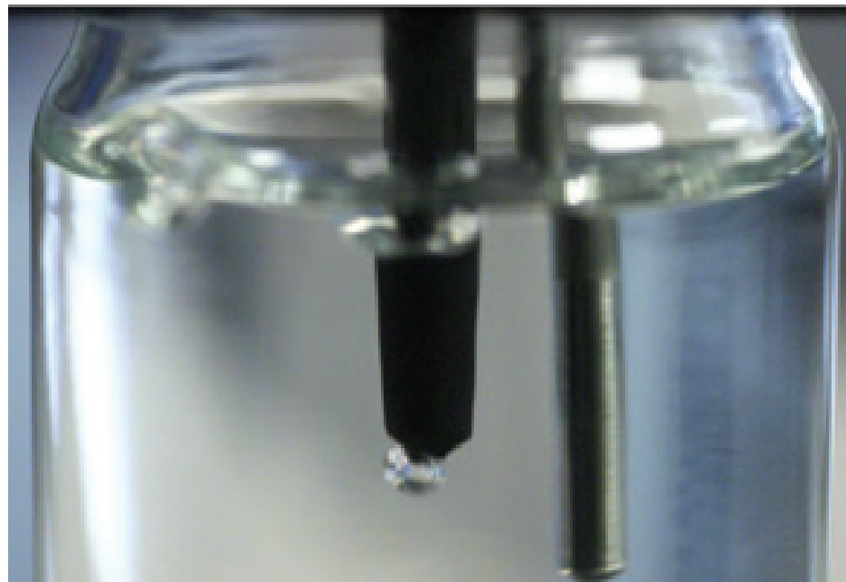
Figure 3: Bubble pressure tensiometer producing a gas bubble in a liquid
