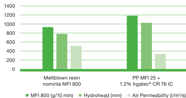
Meltblown by vis-breaking spunbond PP
