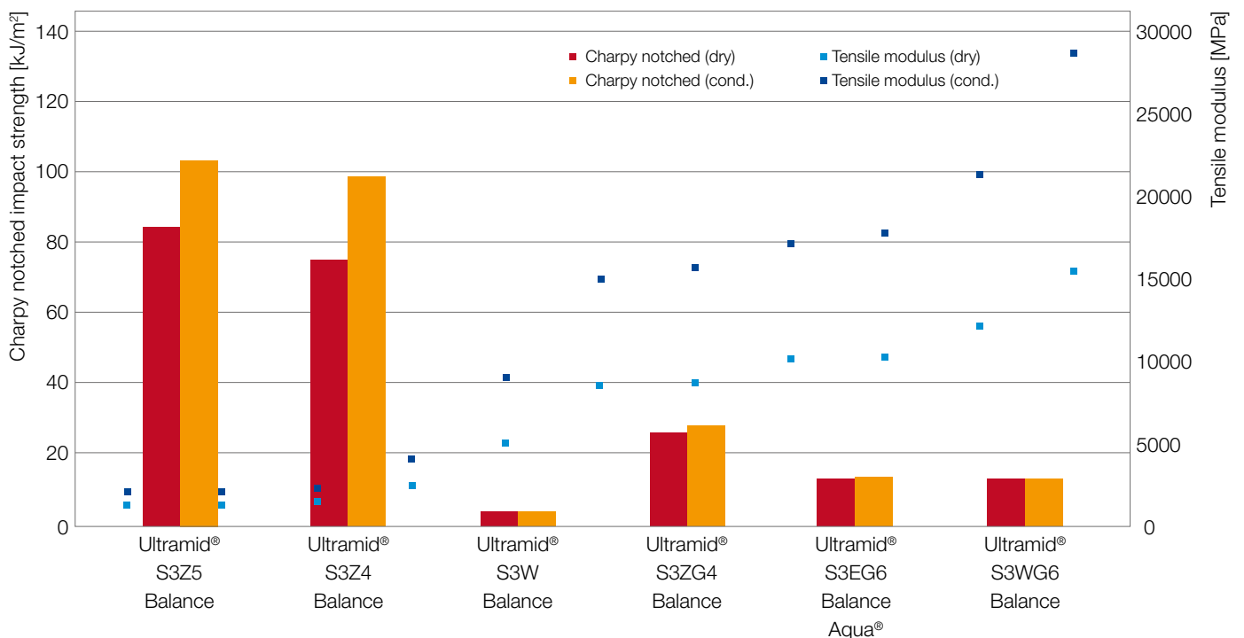
Fig. 8: Stiffness and toughness of Ultramid® S grades
