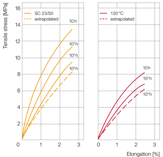
Fig. 20: Isochronous stress-strain curves for Ultramid® A3K in accordance with ISO 899 under standard climate conditions (23 °C/50 % r.h.) and at 120 °C (in the dry state)
