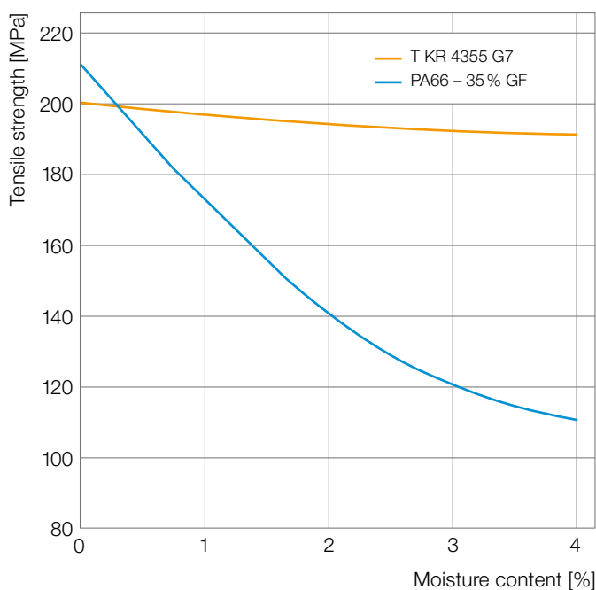
Fig. 1: Tensile strength of Ultramid® T KR compared to PA66 at 23 °C, different moisture contents
