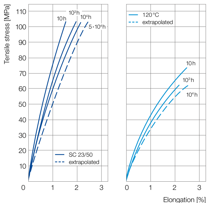
Fig. 21: Isochronous stress-strain curves for Ultramid® A3WG10 in accordance with ISO 899 under standard climate conditions (23 °C/50 % r.h.) and at 120 °C (in the dry state)
