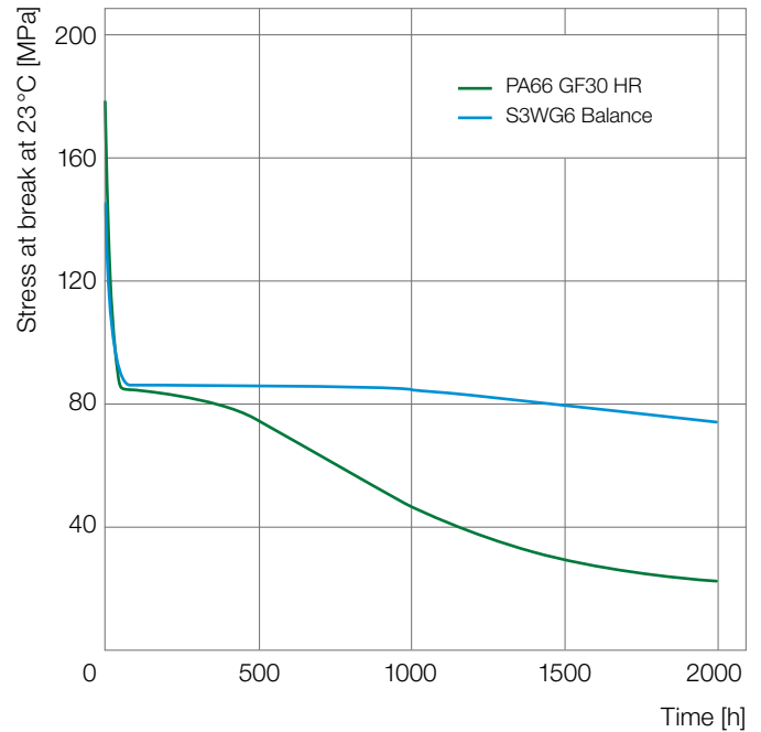
Fig. 7: Hydrolysis resistance of Ultramid® S Balance compared with PA66, in Glystantin®/water (1:1) at 130 °C
