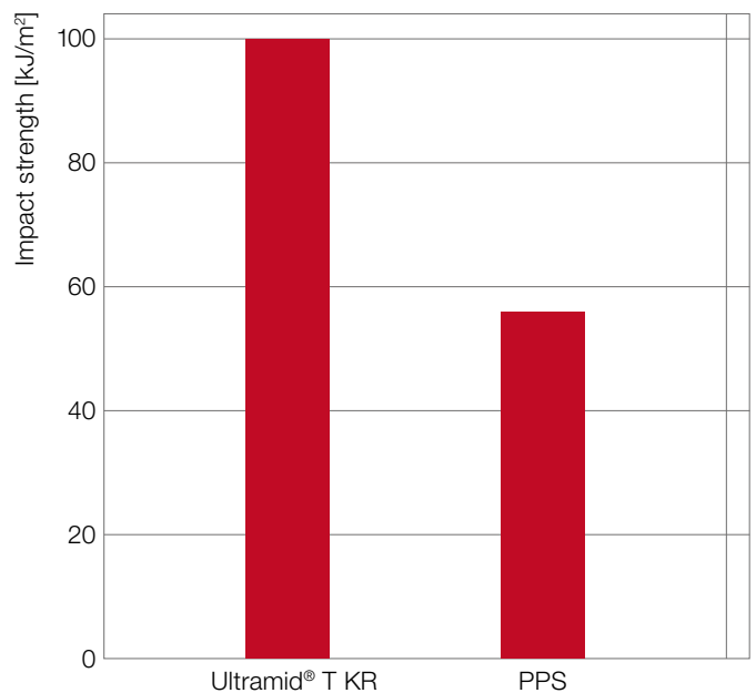
Fig. 2: Impact strength (23 °C) of Ultramid® T KR compared to PPS (glass fiber content: 30-35 %)
