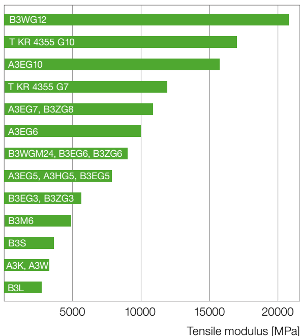
Fig. 12: Tensile modulus for selected Ultramid® grades at 23 °C, dry (ISO 527)
