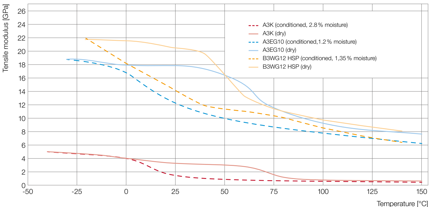
Fig. 10: Tensile modulus for selected Ultramid® grades as function of temperature and conditioning
