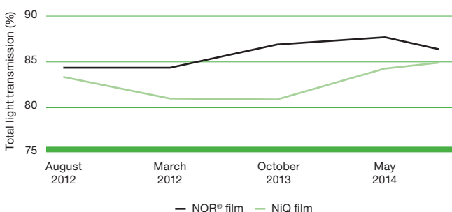
Total light transmission upon weathering (films washed to eliminate white washing effect)
