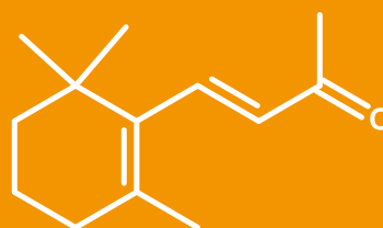
(E)-4-(2,6,6-Trimethyl-1-cyclohexen-1-yl)-3-buten-2-one
