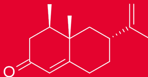
(4R,4aS,6R)-4,4a-dimethyl-6-(prop-1-en-2-yl)-4,4a,5,6,7,8-hexahydronaphthalen2(3H)-one
