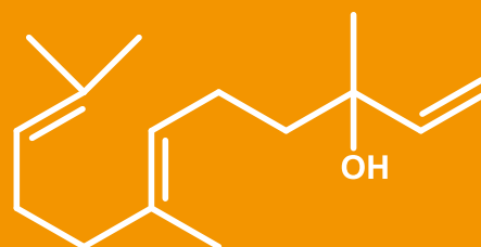
1,6,10-Dodecatrien-3-ol, 3,7,11-trimethyl-
