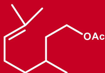
3,7-Dimethyloct-6-en-1-yl acetate
