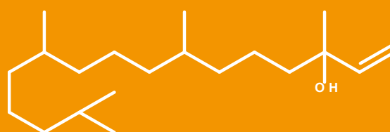
3, 7, 11, 15- Tetramethylhexadec-1-en-3-ol
