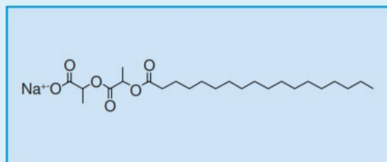
Sodium stearyl-2-lactylate
