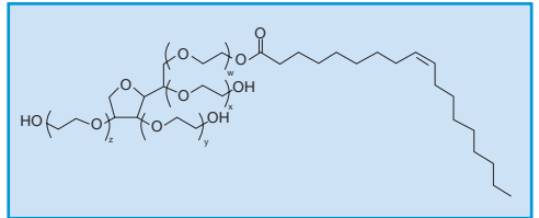
Polyoxyethylene sorbitan monooleate
