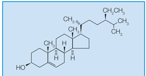
Beta-Sitosterol C_{29}H_{50}O | Molar mass 414.69 g/mol
