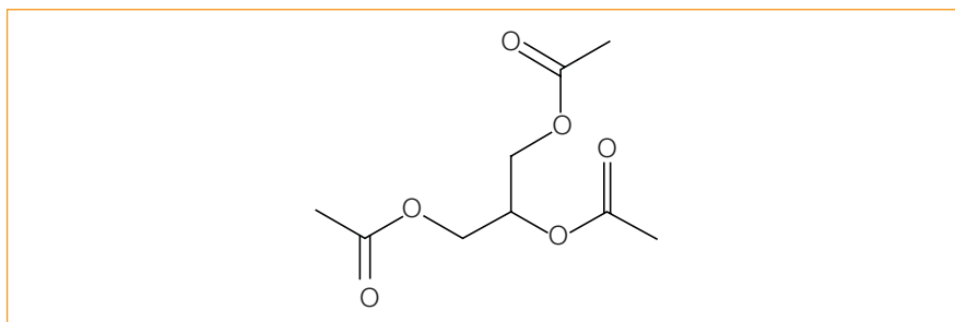
Figure 1: Chemical structure of Triacetin
